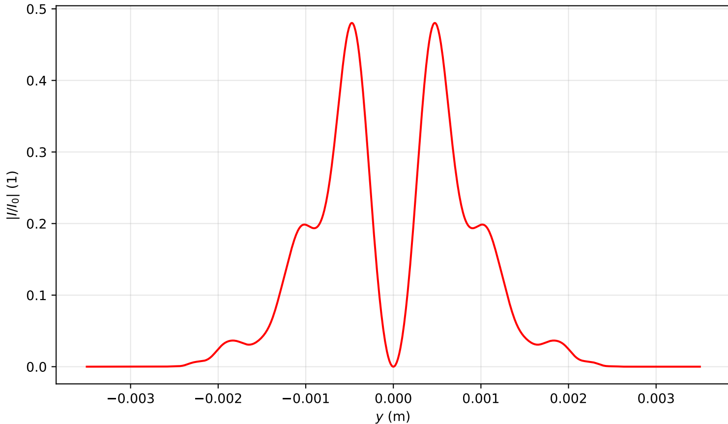
Intensity profile I(x = 0, y, z = 2.548)/I_0 , P_{in}=5.0P_{cr} , artificial time
